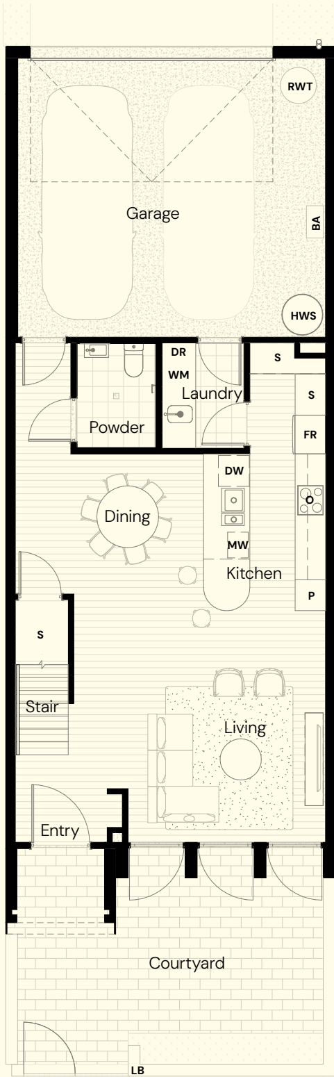
Ground floor
